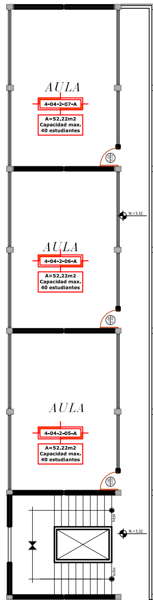
1er PLANTA ALTA ESC: 1/50 AREA=268.26m 2
