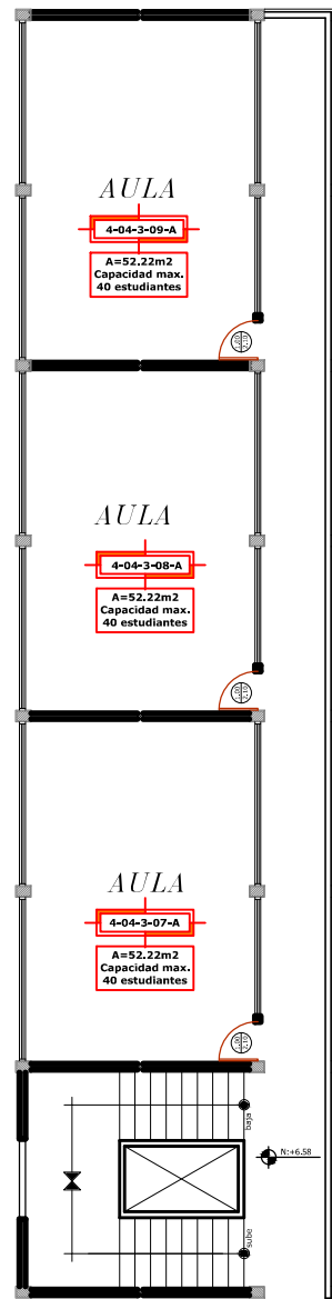
2da PLANTA ALTA ESC: 1/50 AREA=268.26m 2
